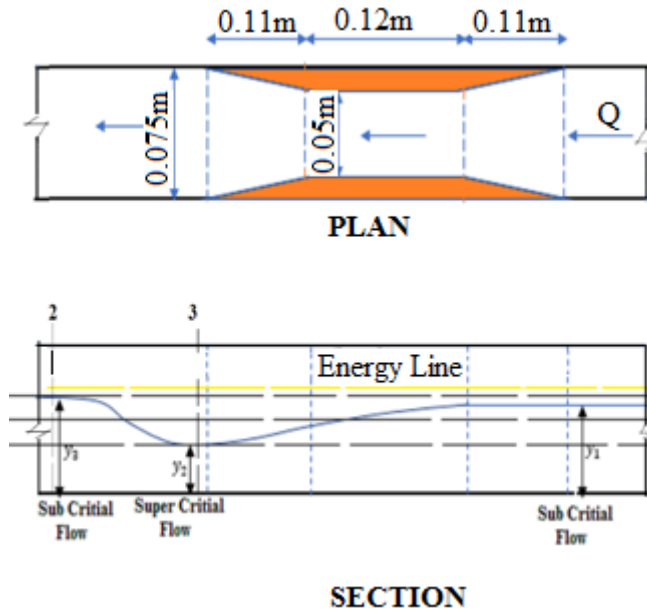
Fig. 7: Flow Through a Constricted Flume
