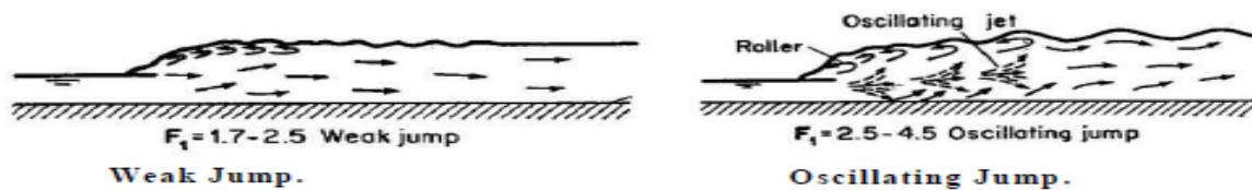
Fig. 10: Classification of Hydraulic Jump. Reprinted From “Experimental Study of Hydraulic Jump In Open Channel: Measurement And Comparison Of Theoretically Predicted Profile” by Lalnunluanga, Examination Roll No. M4MEC13-40 University Registration No. 113533 of 2010 – 11.
