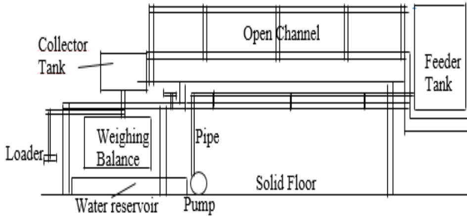
Gravinometric Open Channel Apparatus
